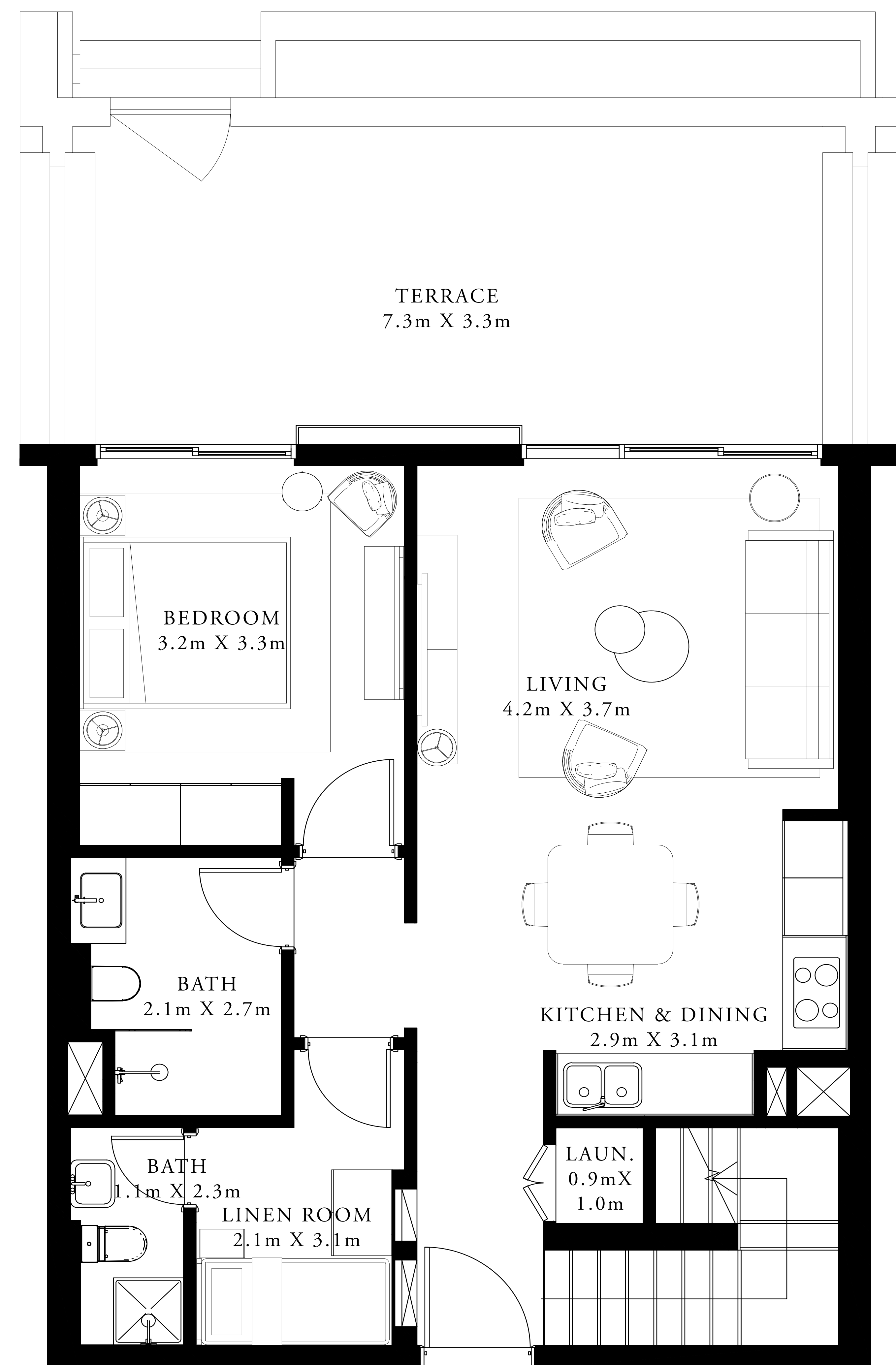
GROUND FLOOR
