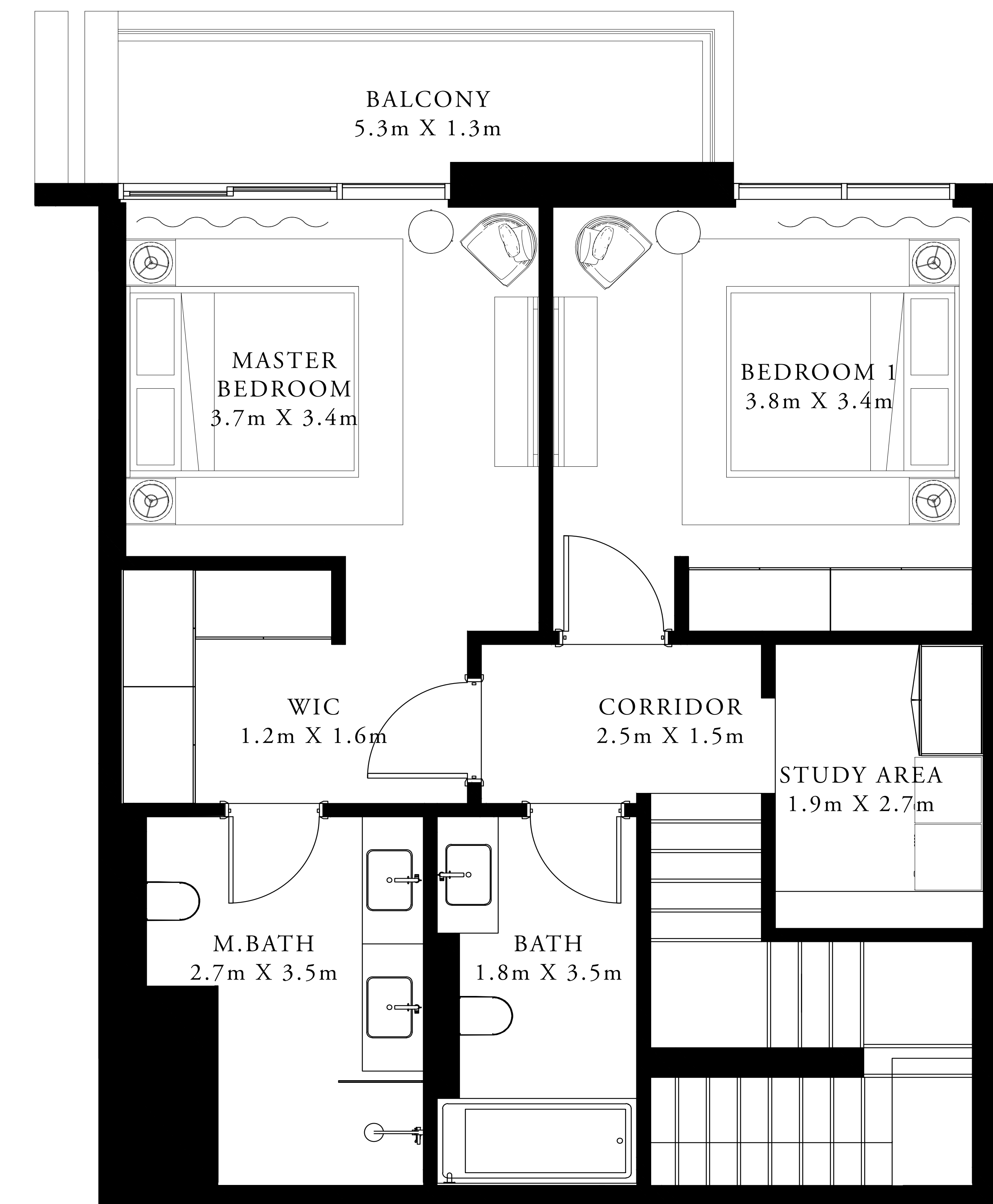
FIRST FLOOR
